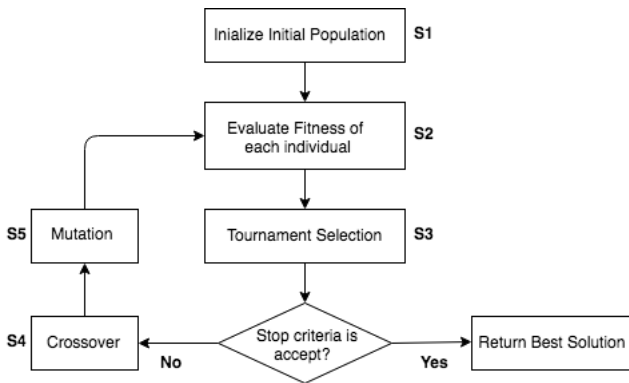
Fig. 5. Genetic algorithm diagram.
